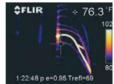
Loose connection on breaker
