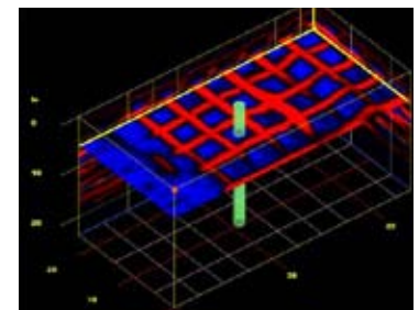
3D image of rebar mat in concrete slab using ground penetrating radar*
