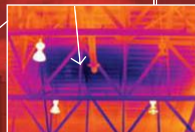
Roof saturated with moisture
