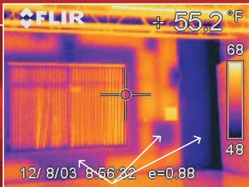
Missing insulation in pre-cast panels
